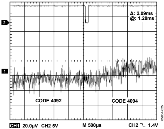
Figure 33. DAC Output with 50 Hz Filter on Output
