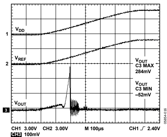
Figure 14. Power-On Reset to 0 V
