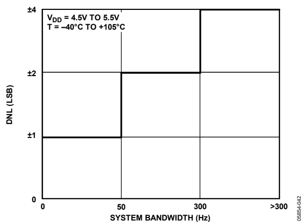
Figure 6. DNL Performance vs. System Bandwidth
