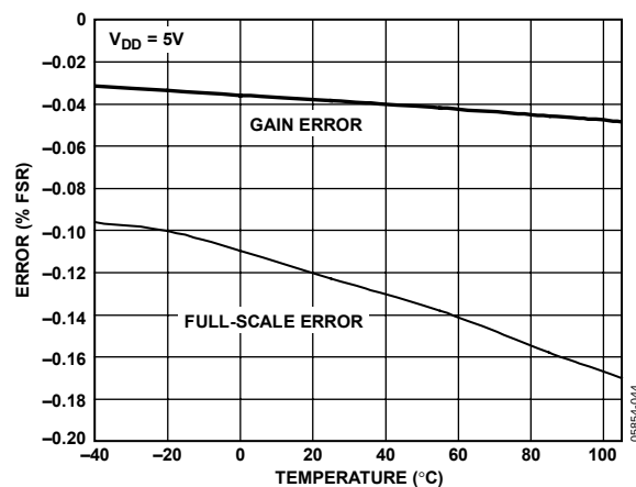
Figure 7. Gain Error and Full-Scale Error vs. Temperature
