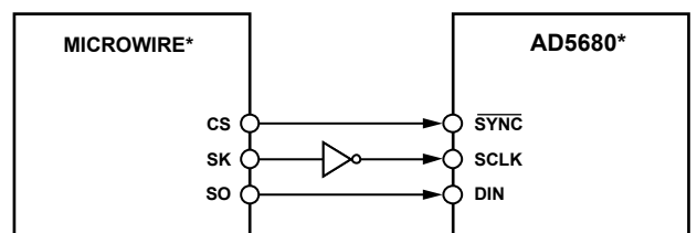
Figure 30. AD5680 to MICROWIRE Interface
