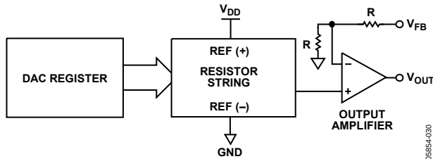
Figure 22. DAC Architecture
