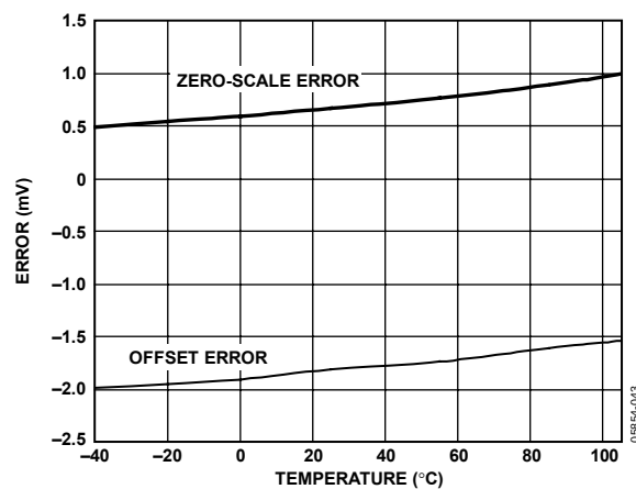
Figure 8. Zero-Scale Error and Offset Error vs. Temperature
