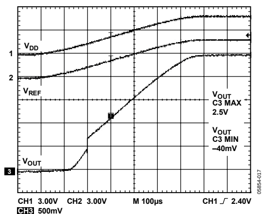
Figure 15. Power-On Reset to Midscale
