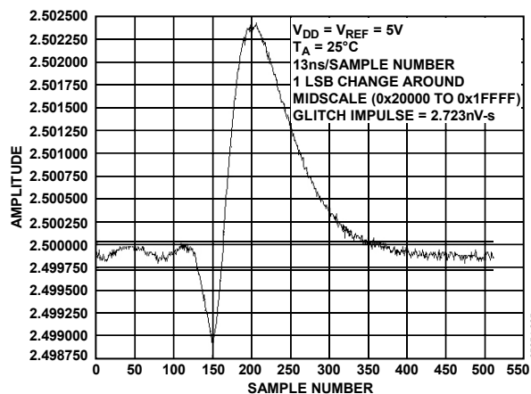
Figure 16. Digital-to-Analog Glitch Impulse (Negative)
