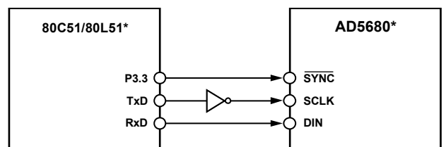
Figure 29. AD5680 to 80C51/80L51 Interface
