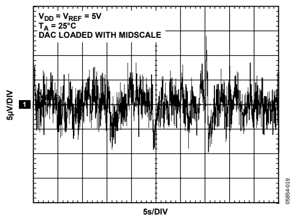
Figure 20. 0.1 Hz to 10 Hz Output Noise Plot
