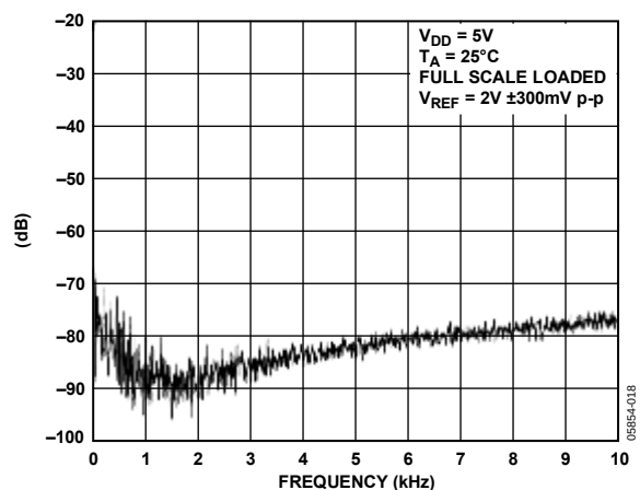
Figure 18. Total Harmonic Distortion
