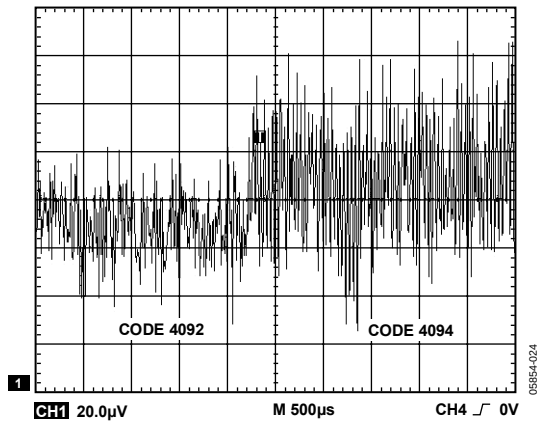
Figure 32. DAC Output Unfiltered
