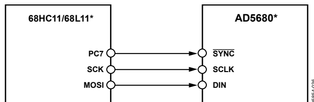
Figure 28. AD5680 to 68HC11/68L11 Interface
