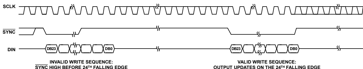
Figure 26. \overline{\text{SYNC}} Interrupt Facility
