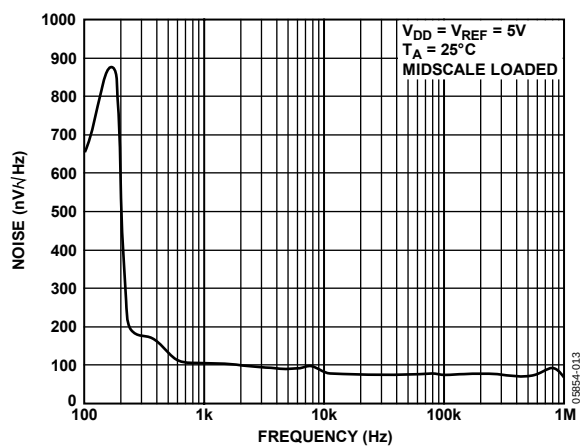
Figure 21. Noise Spectral Density
