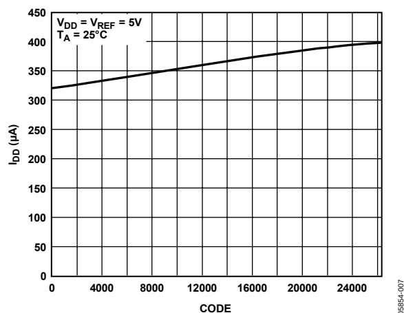
Figure 10. Supply Current vs. Code
