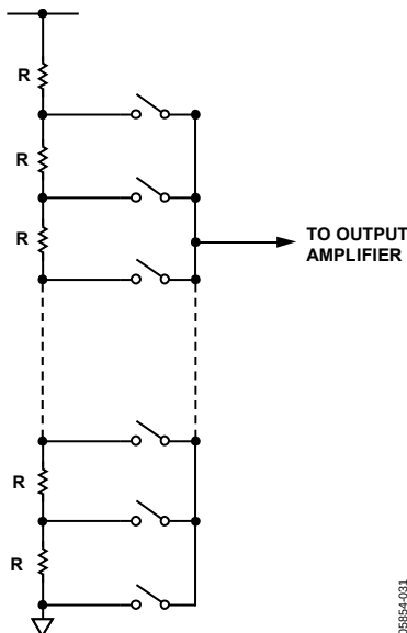
Figure 23. Resistor String
