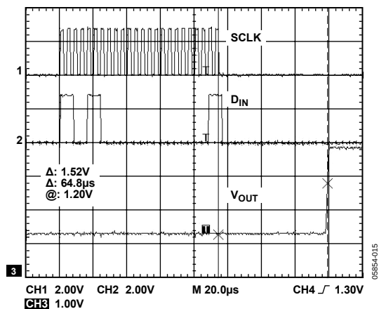
Figure 13. Full-Scale Settling Time, 5 V
