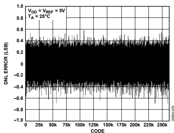
Figure 5. Typical DNL Plot in 50 Hz System Bandwidth
