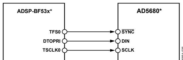
Figure 27. AD5680 to Blackfin ADSP-BF53x Interface
