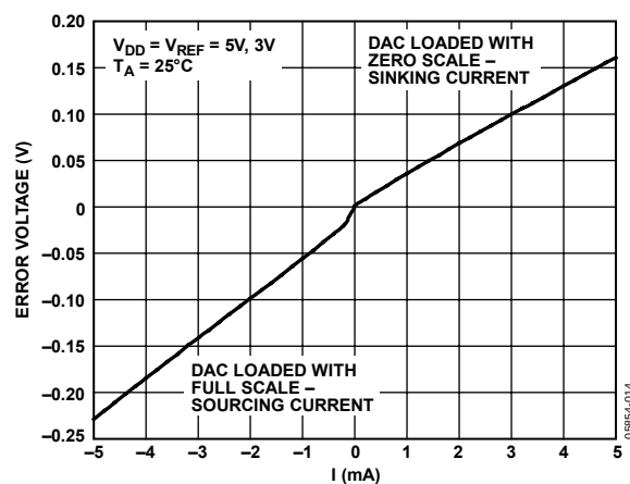
Figure 9. Headroom at Rails vs. Source and Sink Current
