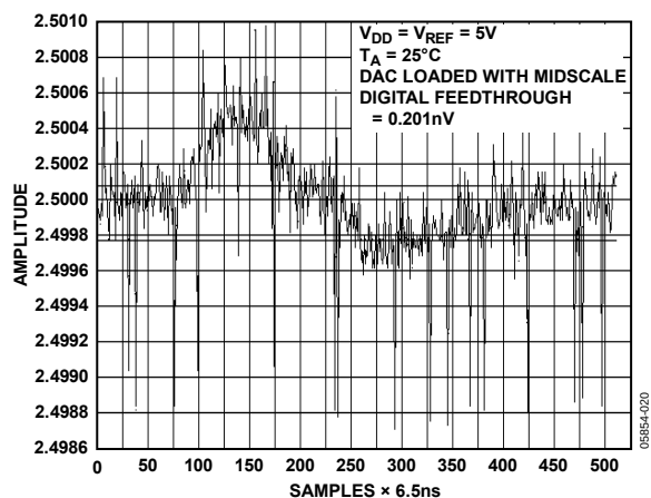
Figure 17. Digital Feedthrough
