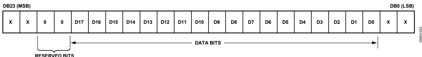
Figure 25. Input Register Contents
