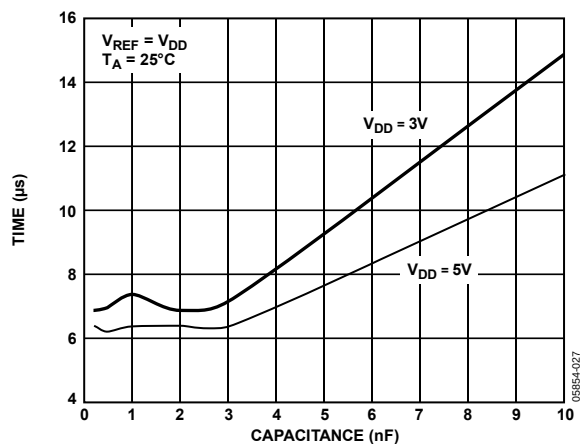
Figure 19. Settling Time vs. Capacitive Load
