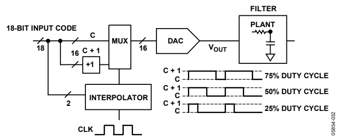
Figure 24. Interpolation Architecture
