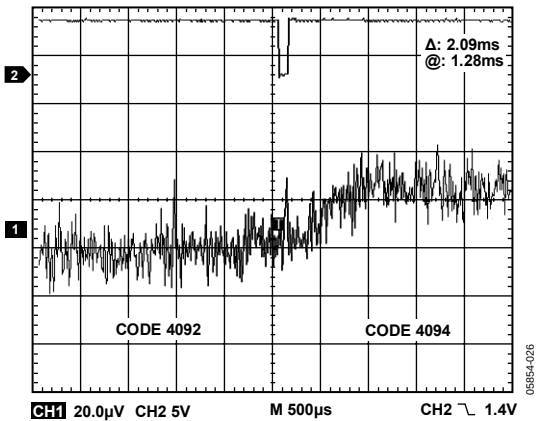
Figure 34. DAC Output with 300 Hz Filter on Output
