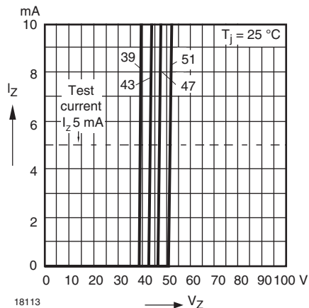
Fig. 14 - Breakdown Characteristics
