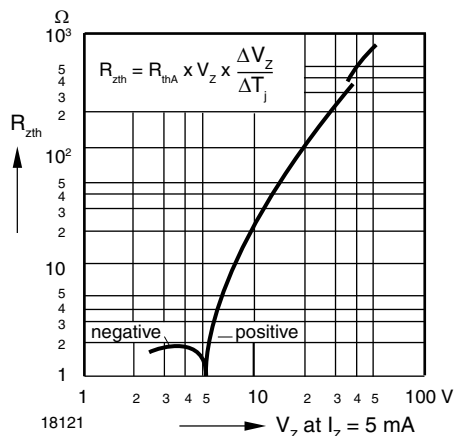
Fig. 4 - Thermal Differential Resistance vs. Zener Voltage
