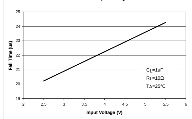
Fall Time vs Input Voltage
