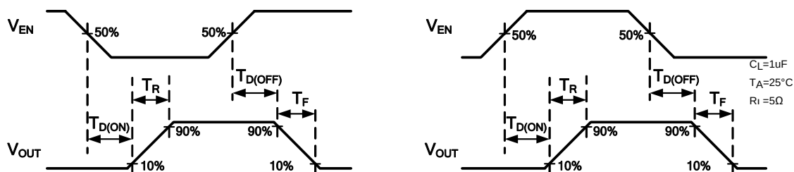
Figure 1. Voltage Waveforms: AP2186 (left), AP2196 (right)
