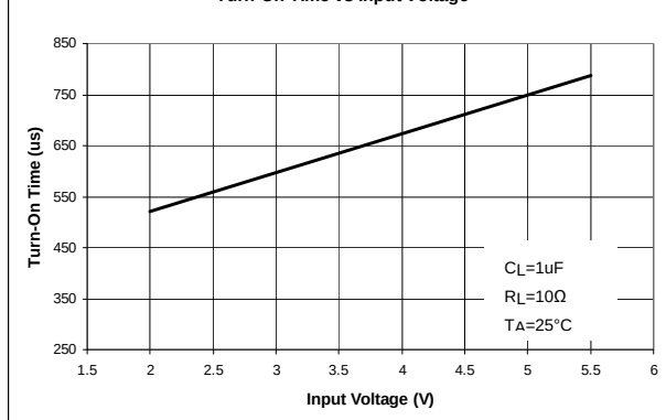
Turn-On Time vs Input Voltage
