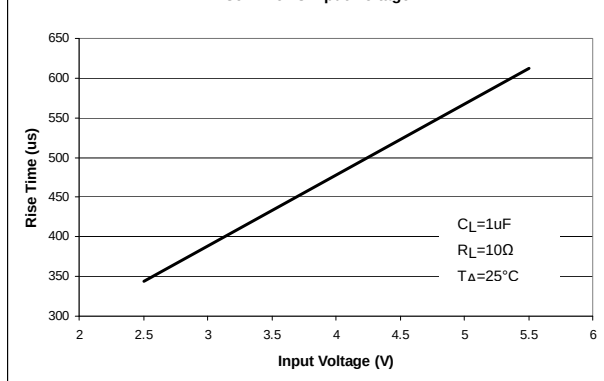
Rise Time vs Input Voltage
