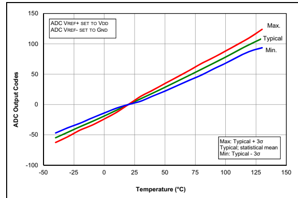
FIGURE 33-92: Temperature Indicator Slope Normalized to 20°C, Low Range, V_{DD} = 3.0V , PIC16LF1705/9 Only.
