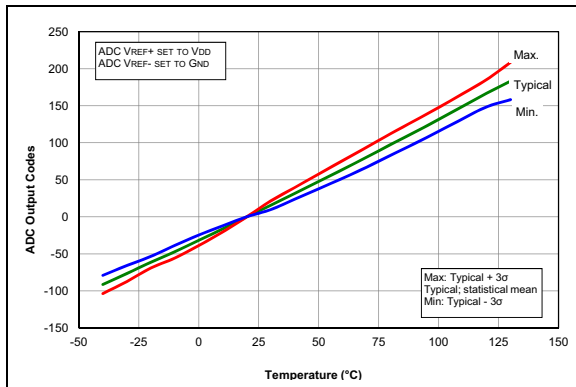
FIGURE 33-93: Temperature Indicator Slope Normalized to 20°C, High Range, V_{DD} = 3.6V , PIC16LF1705/9 Only.
