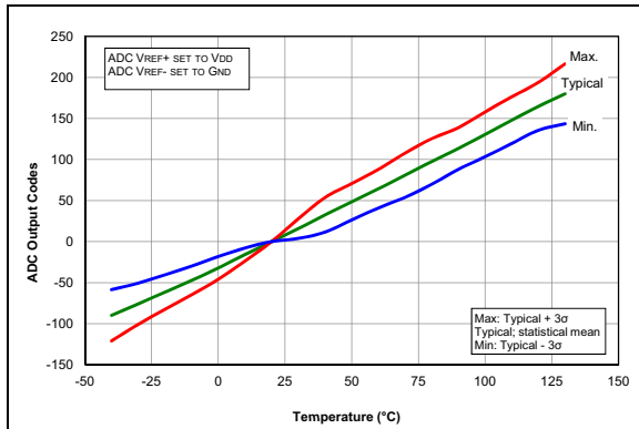
FIGURE 33-91: Temperature Indicator Slope Normalized to 20°C, Low Range, V_{DD} = 1.8V , PIC16LF1705/9 Only.
