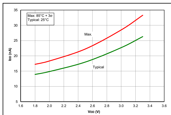
FIGURE 33-37: I_{DD} , Fixed Voltage Reference (FVR), PIC16LF1705/9 Only.
