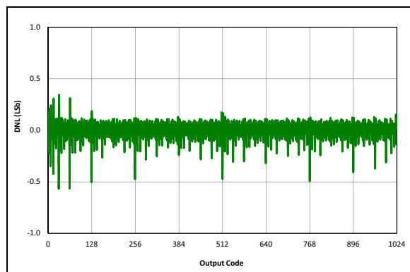
FIGURE 33-77: ADC 10-Bit Mode, Single-Ended DNL, V_{DD} = 3.0V , T_{AD} = 1\text{ }\mu\text{s} , 25^\circ\text{C} .
