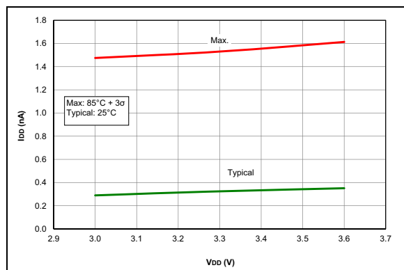
FIGURE 33-41: I_{DD} , LP Brown-Out Reset ( LPBOR = 0 ), PIC16LF1705/9 Only.
