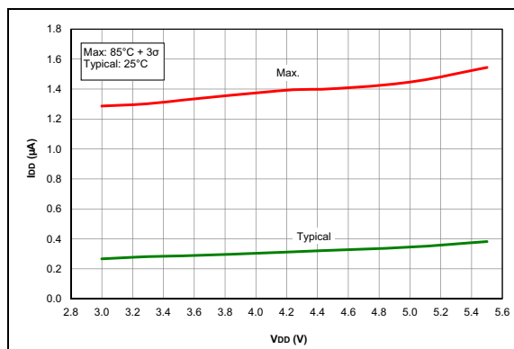
FIGURE 33-42: I_{DD} , LP Brown-Out Reset ( LPBOR = 0 ), PIC16F1705/9 Only.
