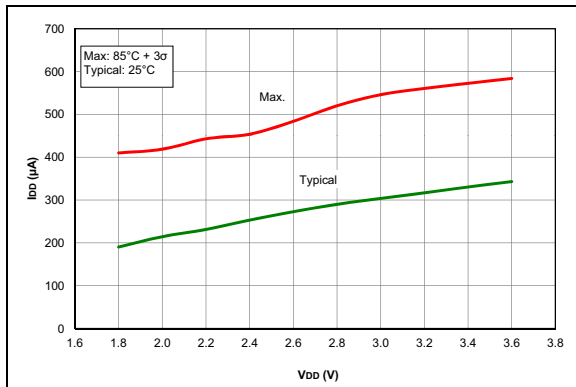
FIGURE 33-45: I_D , Op Amp, High GBWP Mode ( OPAxSP = 1 ), PIC16LF1705/9 Only.
