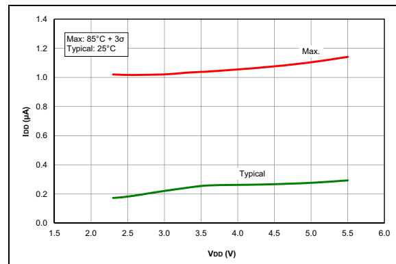
FIGURE 33-48: I_D , ADC Non-Converting, PIC16F1705/9 Only.
