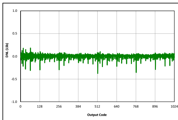
FIGURE 33-78: ADC 10-Bit Mode, Single-Ended DNL, V_{DD} = 3.0V , T_{AD} = 4\text{ }\mu\text{s} , 25^\circ\text{C} .
