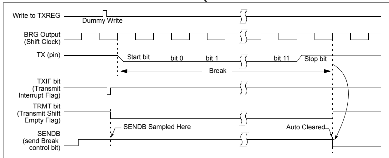
FIGURE 29-9: SEND BREAK CHARACTER SEQUENCE
