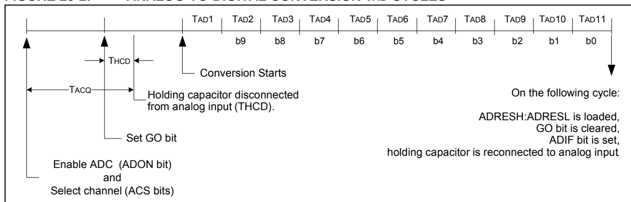
FIGURE 20-2: ANALOG-TO-DIGITAL CONVERSION T AD CYCLES
