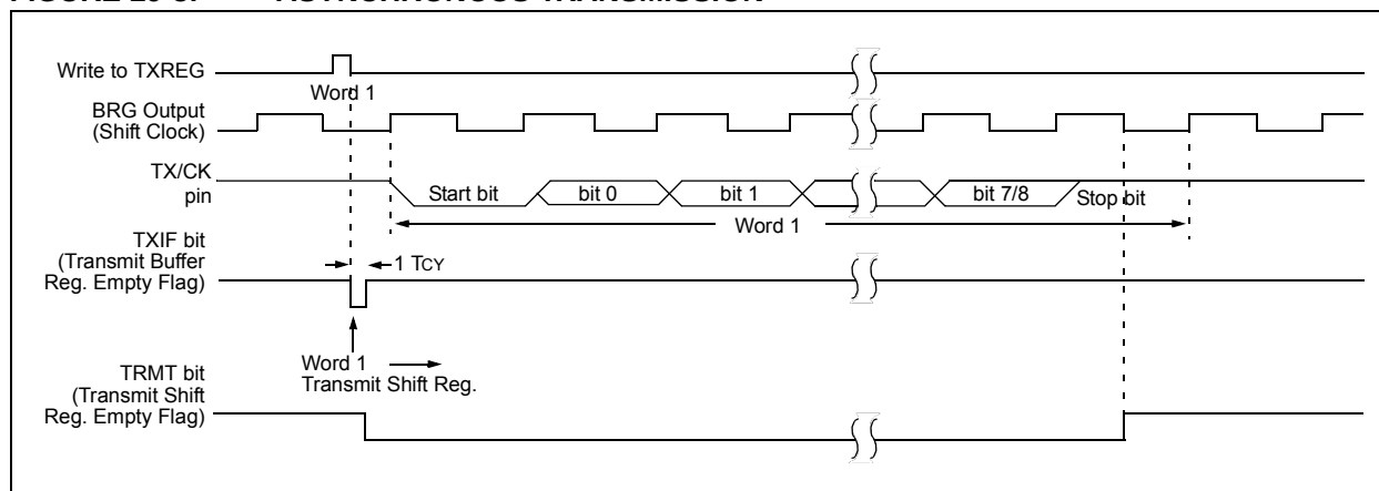
FIGURE 29-3: ASYNCHRONOUS TRANSMISSION
