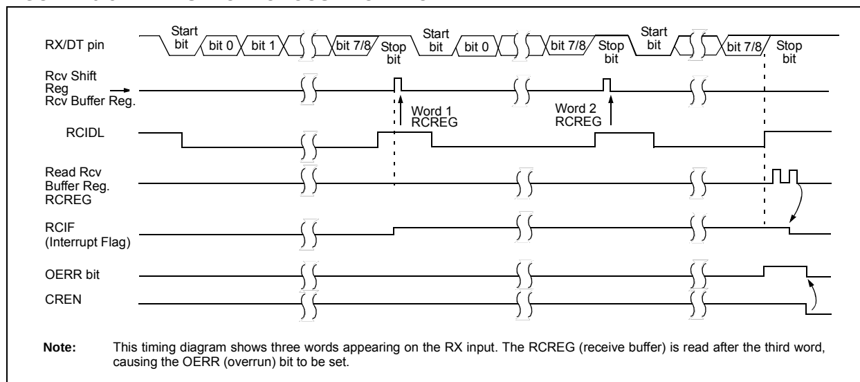
FIGURE 29-5: ASYNCHRONOUS RECEPTION
