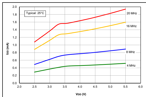
FIGURE 33-29: I_{DD} Typical, HS Oscillator, 25°C, PIC16F1705/9 Only.
