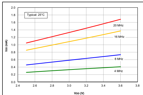
FIGURE 33-27: I_{DD} Typical, HS Oscillator, 25°C, PIC16LF1705/9 Only.
