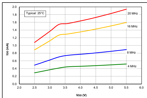
FIGURE 33-29: I_{DD} Typical, HS Oscillator, 25^\circ\text{C} , PIC16F1705/9 Only.
