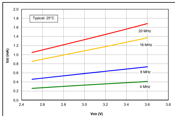
FIGURE 33-27: I_{DD} Typical, HS Oscillator, 25^\circ\text{C} , PIC16LF1705/9 Only.
