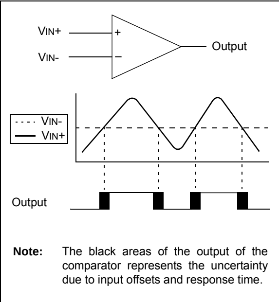
FIGURE 16-1: SINGLE COMPARATOR
