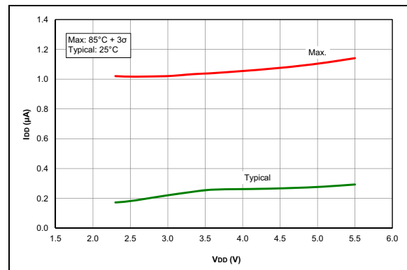
FIGURE 33-48: I_{PD} , ADC Non-Converting, PIC16F1705/9 Only.
