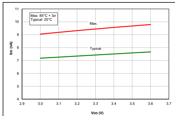
FIGURE 33-39: I_{PD} , Brown-Out Reset (BOR), BORV = 1 , PIC16LF1705/9 Only.
