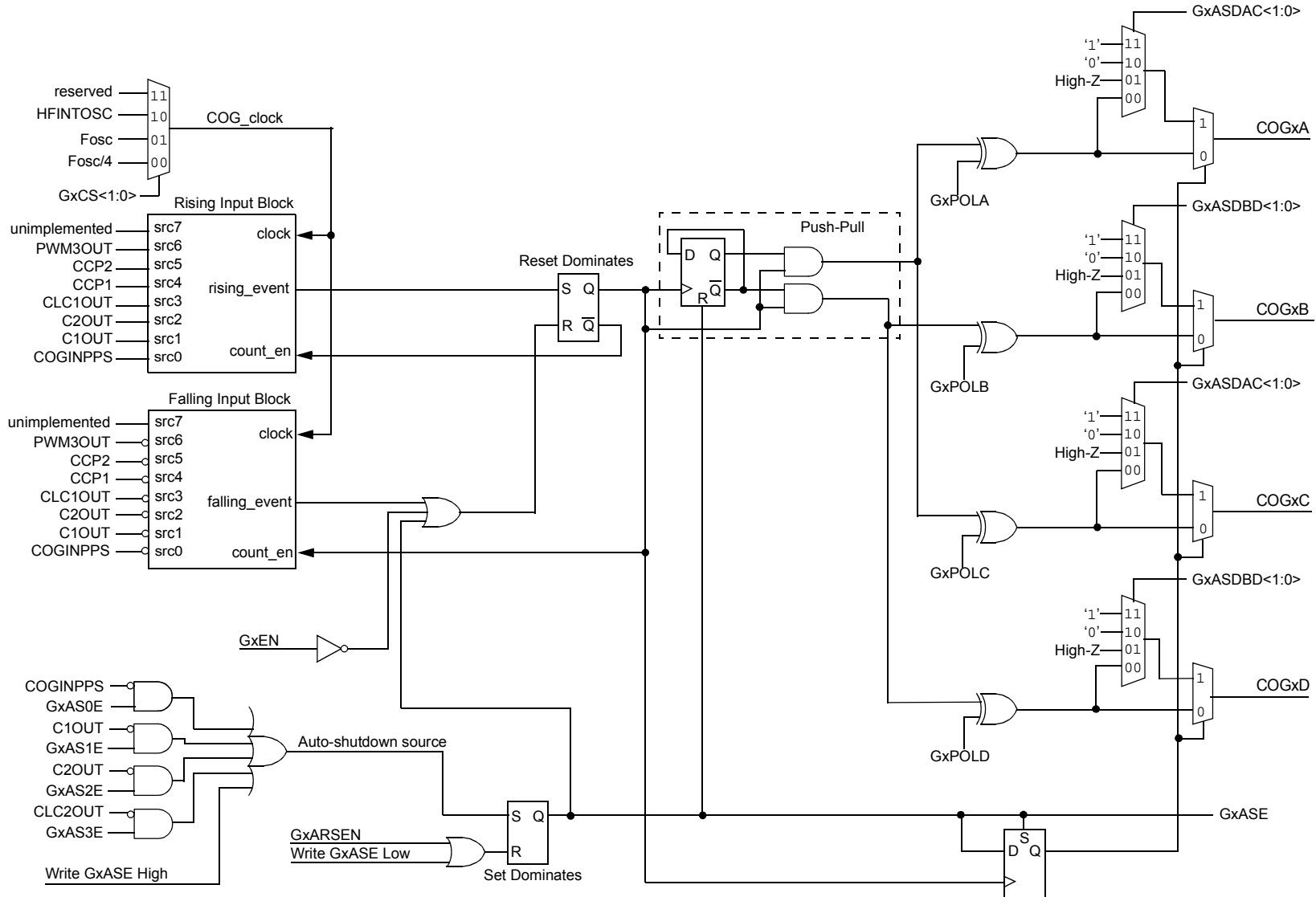
FIGURE 18-6: SIMPLIFIED COG BLOCK DIAGRAM (PUSH-PULL MODE, GXMD = 5)
