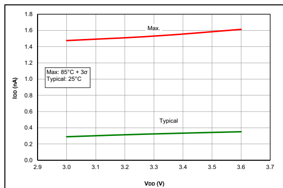
FIGURE 33-41: I_{PD} , LP Brown-Out Reset ( LPBOR = 0 ), PIC16LF1705/9 Only.
