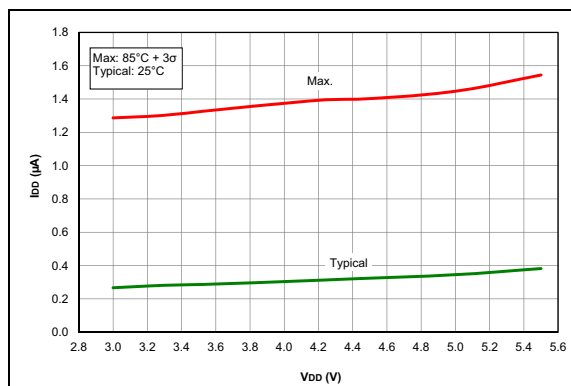
FIGURE 33-42: I_{PD} , LP Brown-Out Reset ( LPBOR = 0 ), PIC16F1705/9 Only.
