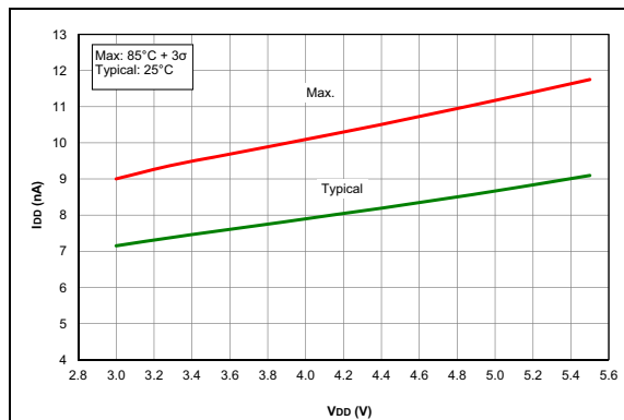
FIGURE 33-40: I_{PD} , Brown-Out Reset (BOR), BORV = 1 , PIC16F1705/9 Only.
