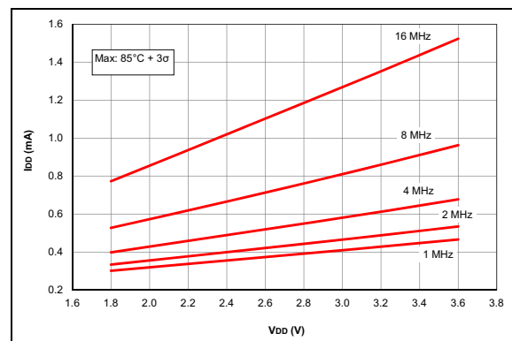
FIGURE 33-24: I_{DD} Maximum, HFINTOSC Mode, PIC16LF1705/9 Only.
