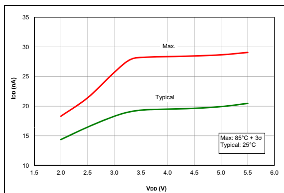
FIGURE 33-38: I_{PD} , Fixed Voltage Reference (FVR), PIC16F1705/9 Only.
