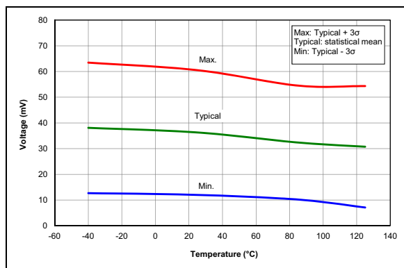
FIGURE 33-66: Brown-Out Reset Hysteresis, High Trip Point (BORV = 0).
