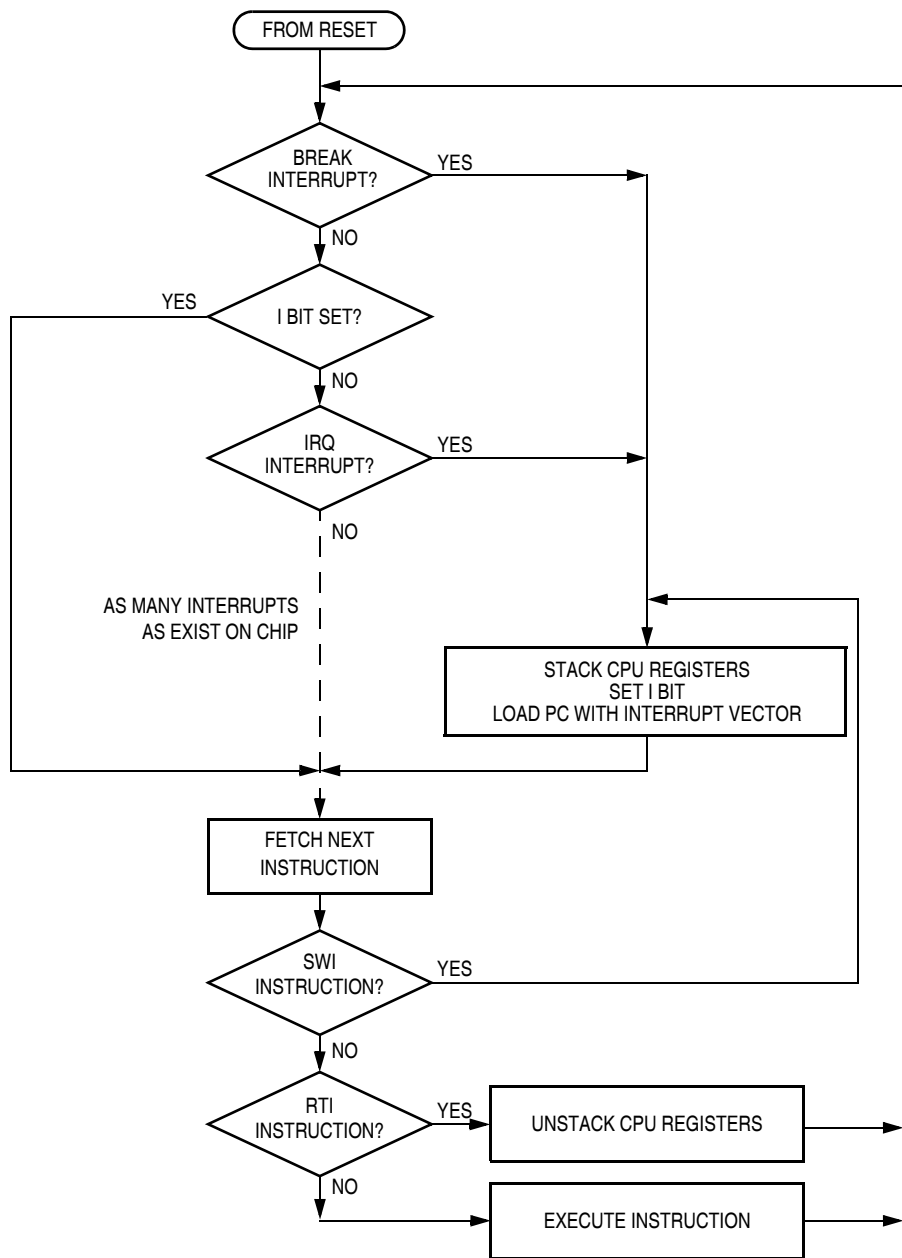
Figure 15-11. Interrupt Processing
