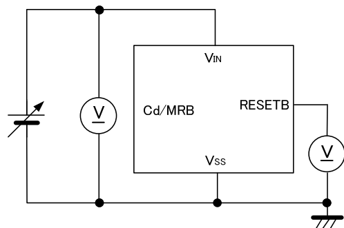
CIRCUIT⑧
