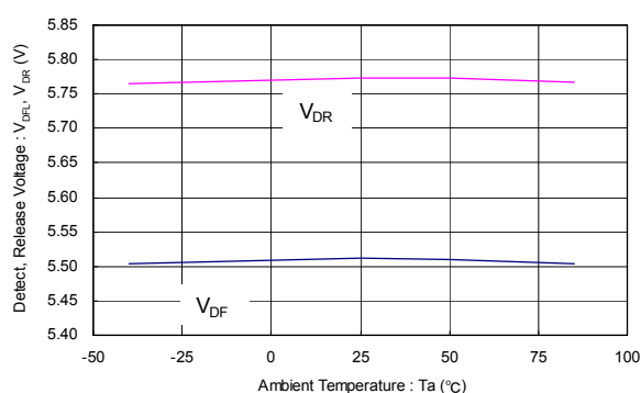
XC6129 ( V_{DF(T)}=5.5V )
