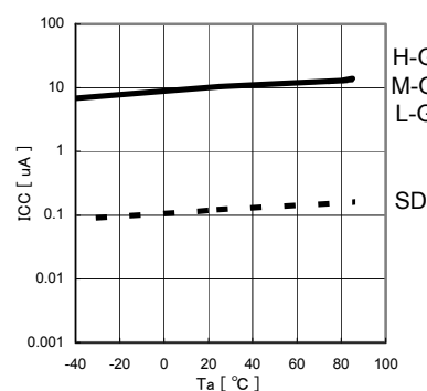
Fig.7 Ta – ICC (0 lx)
