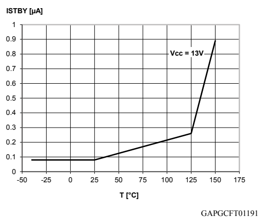
Figure 16. Standby current
