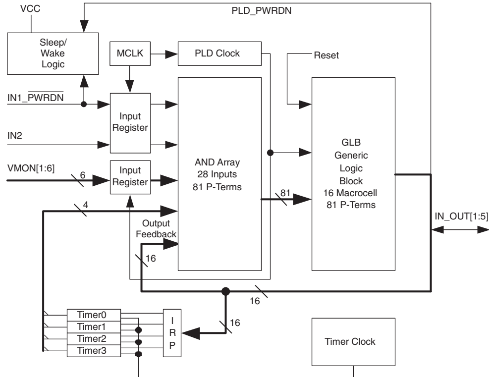
Figure 12. ProcessorPM-POWR605 PLD Architecture
