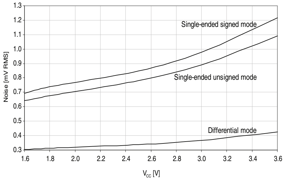
Figure 38-47.Noise vs. V_{CC} .
