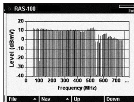
Remote view of Scan Graph on a DSAM
