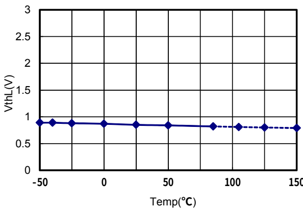
VthL vs Temp
