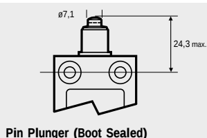
Pin Plunger (Boot Sealed)
