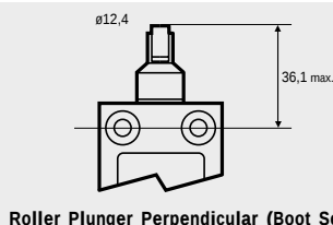
Roller Plunger Perpendicular (Boot Sealed)
