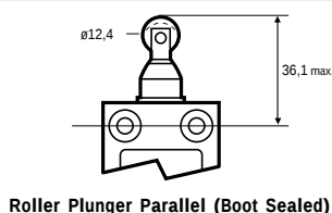
Roller Plunger Parallel (Boot Sealed)
