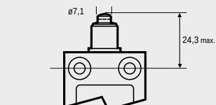
Pin Plunger (Boot Sealed)
