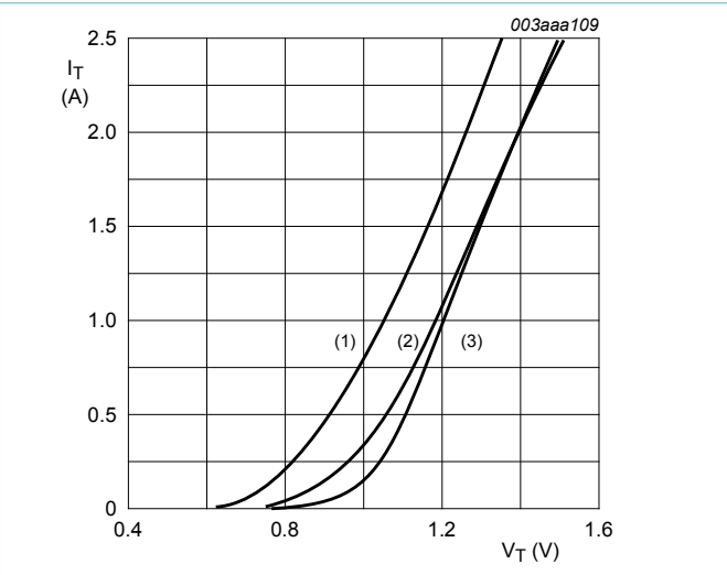
Fig. 10. On-state current as a function of on-state voltage V_o = 0.895 \text{ V}; R_s = 0.195 \Omega (1) T_j = 125 \text{ }^\circ\text{C} ; typical values (2) T_j = 125 \text{ }^\circ\text{C} ; maximum values (3) T_j = 25 \text{ }^\circ\text{C} ; maximum values
