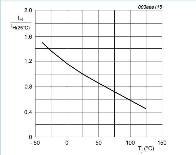
Fig. 9. Normalized holding current as a function of junction temperature R_{GK} = 1 \text{ k}\Omega
