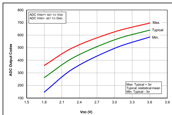
FIGURE 33-87: Temperature Indicator Initial Offset, Low Range, Temp. = 20^\circ C , PIC16LF1704/8 Only.
