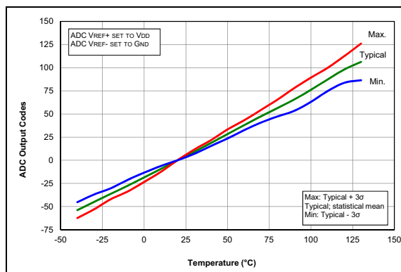
FIGURE 33-90: Temperature Indicator Slope Normalized to 20^\circ C , Low Range, V_{DD} = 3.0V , PIC16F1704/8 Only.
