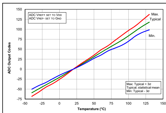
FIGURE 33-88: Temperature Indicator Slope Normalized to 20^\circ C , High Range, V_{DD} = 5.5V , PIC16LF1704/8 Only.
