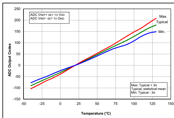
FIGURE 33-89: Temperature Indicator Slope Normalized to 20^\circ C , High Range, V_{DD} = 3V , PIC16F1704/8 Only.
