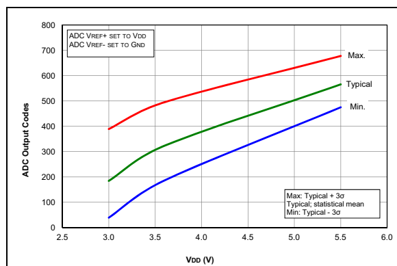
FIGURE 33-85: Temperature Indicator Initial Offset, High Range, Temp. = 20^\circ C , PIC16F1704/8 Only.
