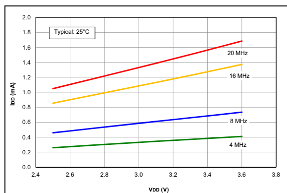
FIGURE 33-27: I_{DD} Typical, HS Oscillator, 25^\circ C . PIC16F1704/8 Only.
