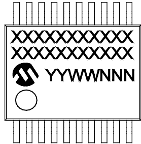
20-Lead SSOP (5.30 mm)
