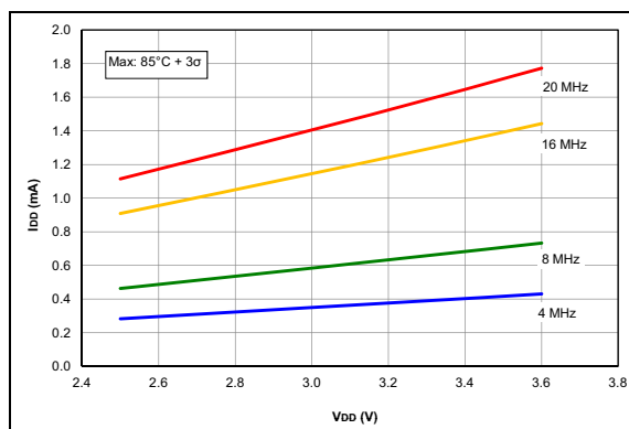
FIGURE 33-28: I_{DD} Maximum, HS Oscillator. PIC16F1704/8 Only.
