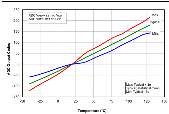
FIGURE 33-91: Temperature Indicator Slope Normalized to 20°C, Low Range, V_{DD} = 1.8V , PIC16LF1704/8 Only.
