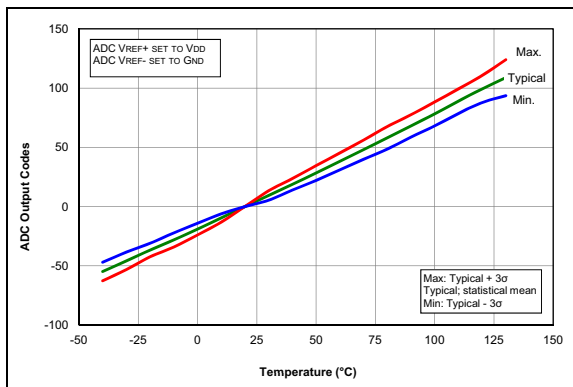
FIGURE 33-92: Temperature Indicator Slope Normalized to 20°C, Low Range, V_{DD} = 3.0V , PIC16LF1704/8 Only.
