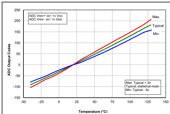
FIGURE 33-93: Temperature Indicator Slope Normalized to 20°C, High Range, V_{DD} = 3.6V , PIC16LF1704/8 Only.
