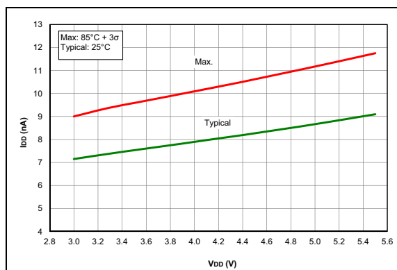
FIGURE 33-40: I_{DD} , Brown-out Reset (BOR), BORV = 1 . PIC16LF1704/8 Only.
