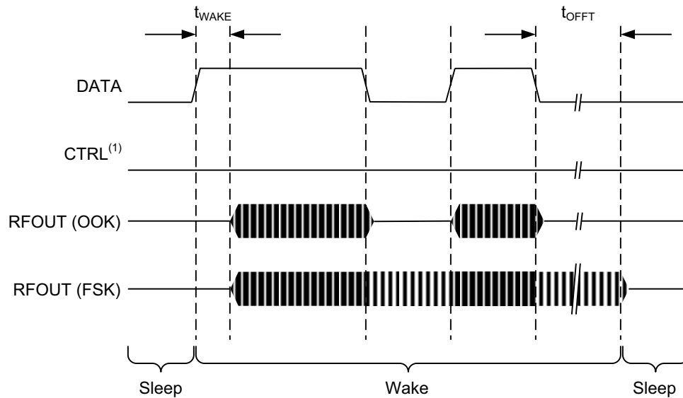
FIGURE 9-5: DATA PIN TRANSMIT TIMING DIAGRAM
