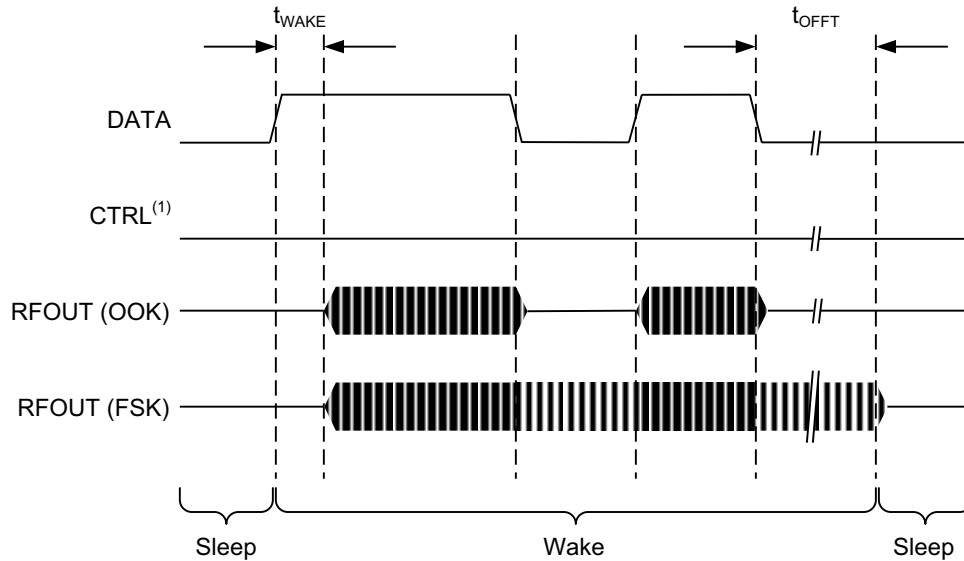
FIGURE 9-5: DATA PIN TRANSMIT TIMING DIAGRAM
