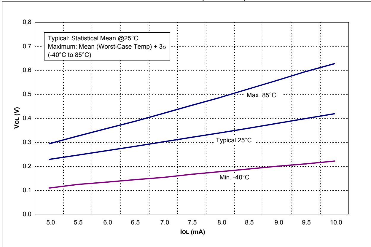
FIGURE 13-9: V OL vs. I OL OVER TEMPERATURE (V DD = 3.0V)
