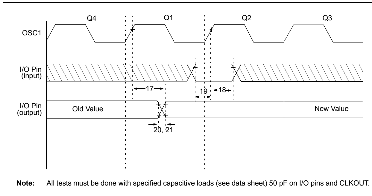
FIGURE 12-5: I/O TIMING
