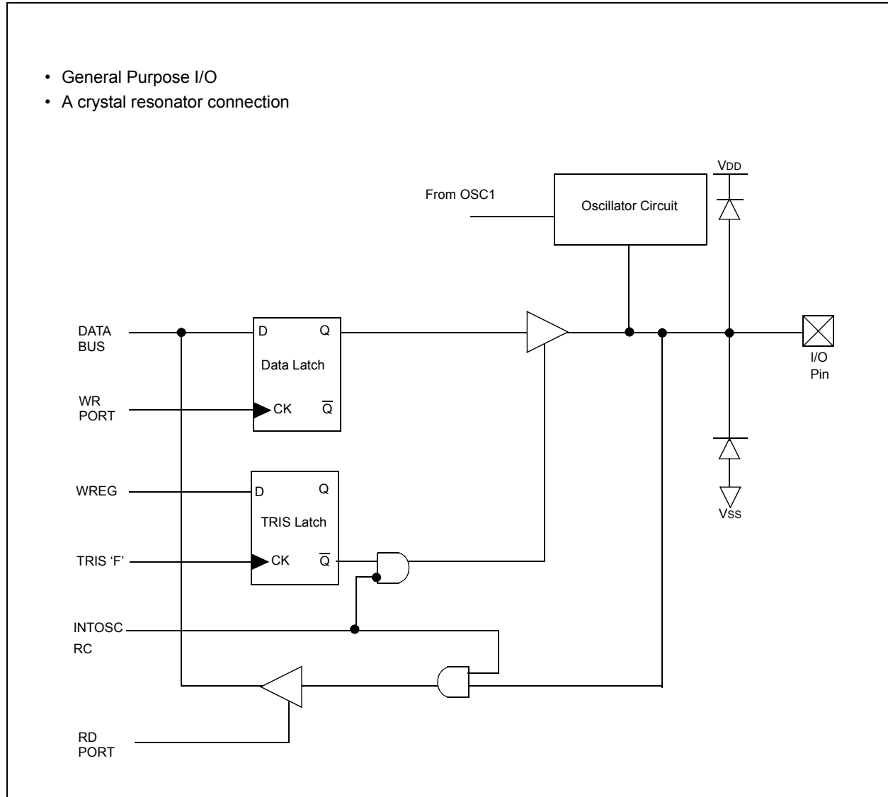
FIGURE 6-3: GP4/OSC2
