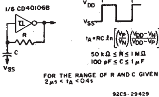
Fig. 18 - Astable multivibrator.
