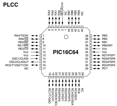
PLCC
