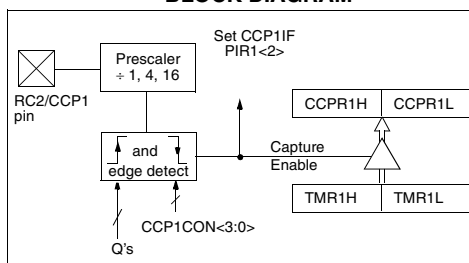
FIGURE 10-2: CAPTURE MODE OPERATION BLOCK DIAGRAM
