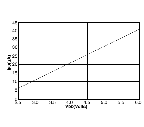
FIGURE 23-11: MAXIMUM I_{PD} vs. TIMER1 ENABLED (32 kHz, RC0/RC1 = 33 pF/33 pF, 85^{\circ}C TO -40^{\circ}C , RC MODE)
