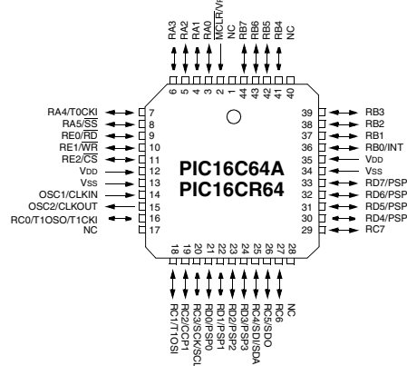
PLCC
