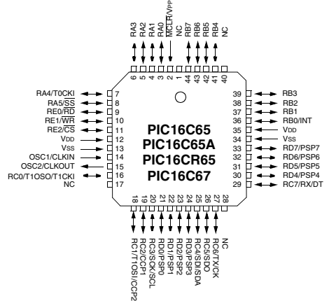
PLCC
