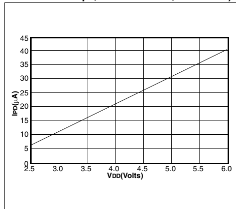
FIGURE 23-11: MAXIMUM I_{PD} vs. TIMER1 ENABLED (32 kHz, RC0/RC1 = 33 \text{ pF}/33 \text{ pF} , 85^{\circ}\text{C} TO -40^{\circ}\text{C} , RC MODE)
