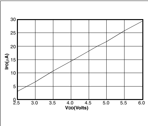
FIGURE 23-11: MAXIMUM I_{PD} vs. TIMER1 ENABLED (32 kHz, RC0/RC1 = 33\text{ pF}/33\text{ pF} , 85^{\circ}C TO -40^{\circ}C , RC MODE)
