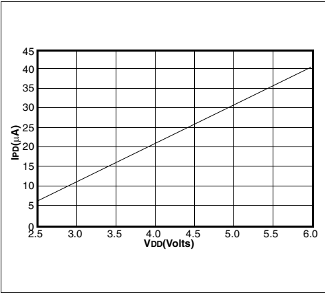
FIGURE 23-11: MAXIMUM I_{PD} vs. TIMER1 ENABLED (32 kHz, RC0/RC1 = 33\text{ pF}/33\text{ pF} , 85^{\circ}C TO -40^{\circ}C , RC MODE)
