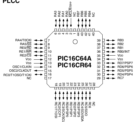
PLCC
