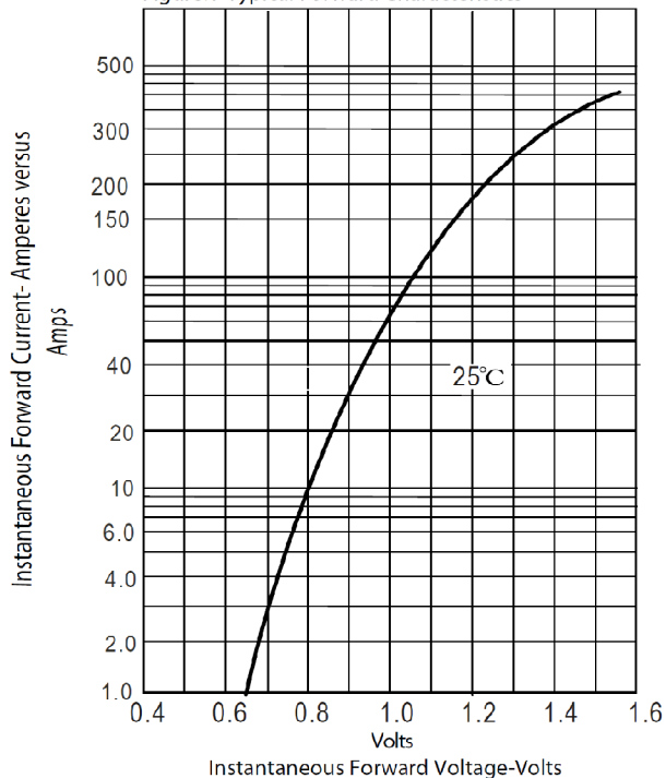
Figure.1-Typical Forward Characteristics
