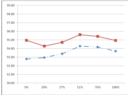
Efficiency at 90 V
