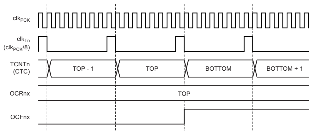
Figure 14-8. Timer/Counter Timing Diagram, CTC mode, with Prescaler ( f_{\text{clk\_IO}}/8 )
