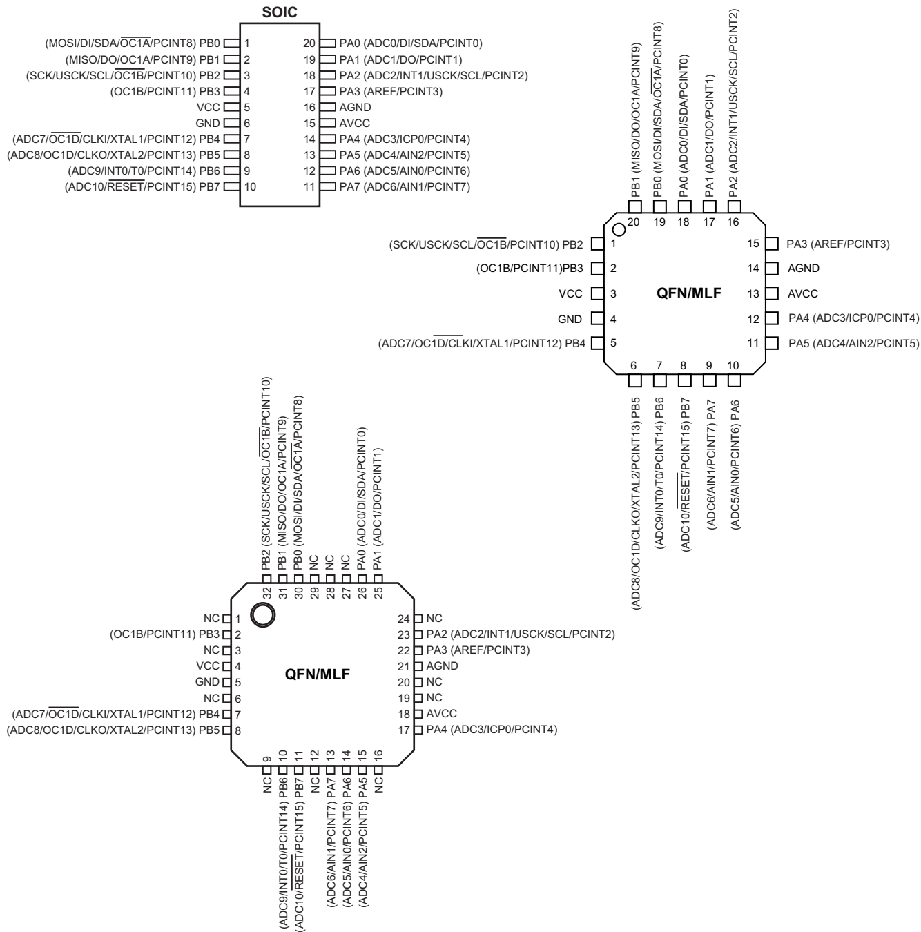
Figure 1-1. Pinout ATtiny261/461/861
