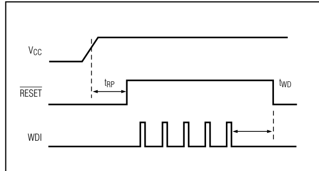
Figure 4. Watchdog Timing
