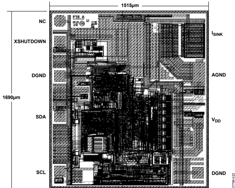
Figure 4. Metallization Photo Dimensions shown in microns (µm)
