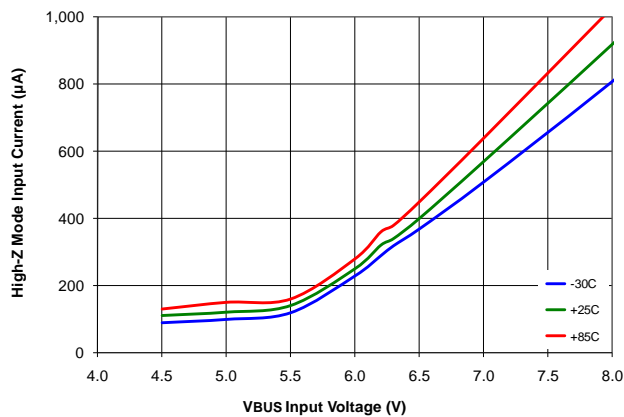
Figure 11. HZ Mode V_{BUS} Current vs. Temperature, 3.7 V BAT
