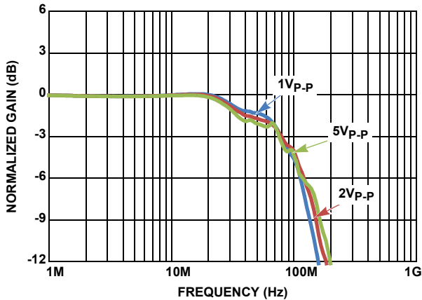
FIGURE 23. LARGE SIGNAL FREQUENCY RESPONSE
