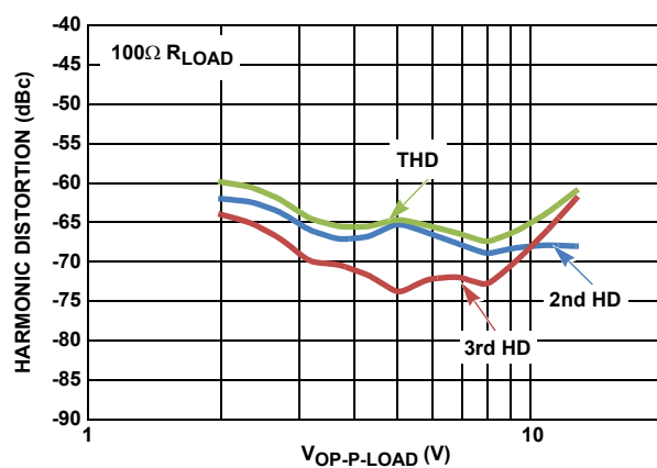
FIGURE 20. 10MHz HARMONIC DISTORTION vs OUTPUT VOLTAGE
