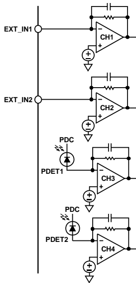
INPUT CONFIGURATION FOR REGISTER 0x14 BITS[11:8] = 5 REGISTER 0x14 BITS[7:4] = 5
