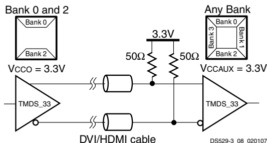
Figure 7: External Input Resistors Required for TMDS_33 I/O Standard
