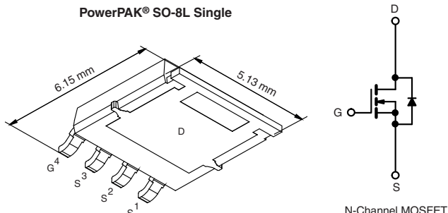
PowerPAK® SO-8L Single
