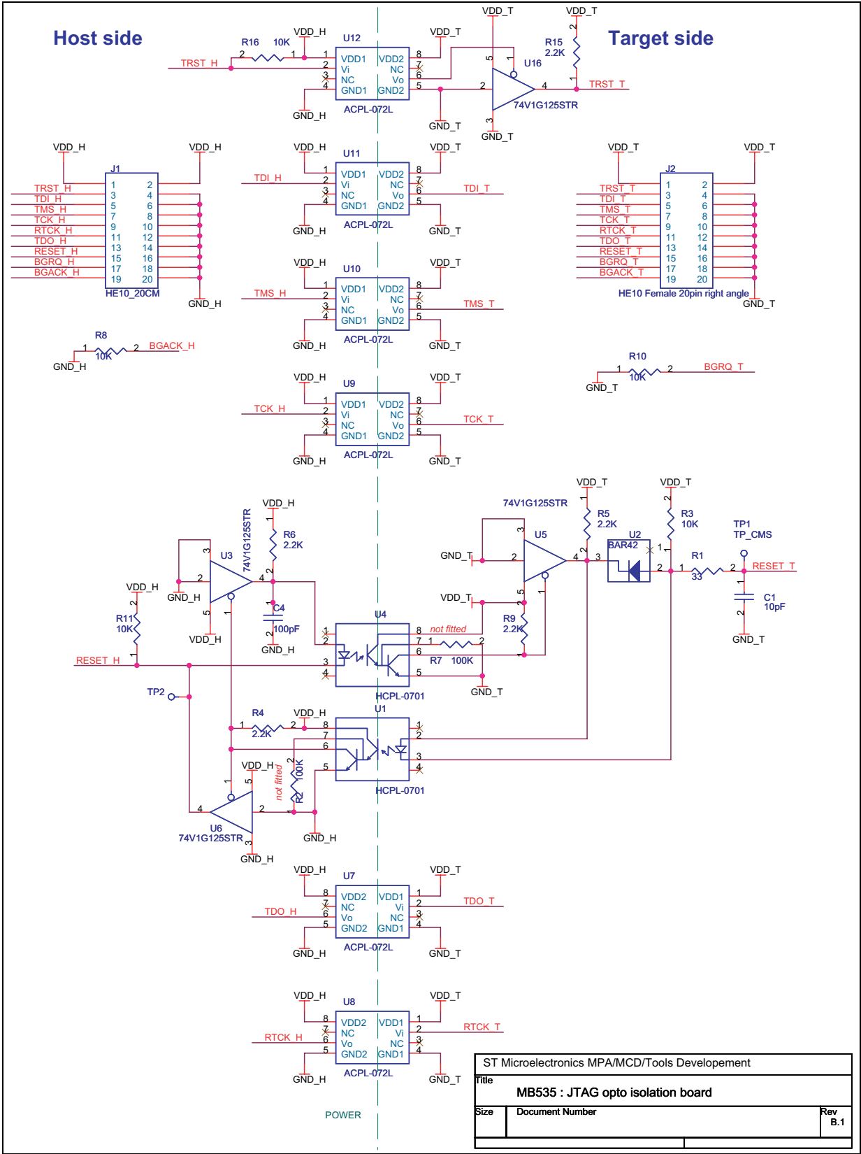
Figure 5. Optocouplers
