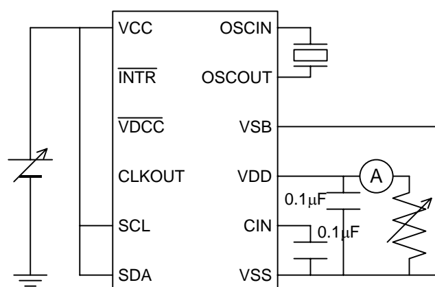
Test circuit
