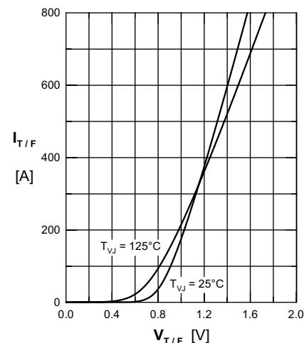
Fig. 1 Forward characteristics
