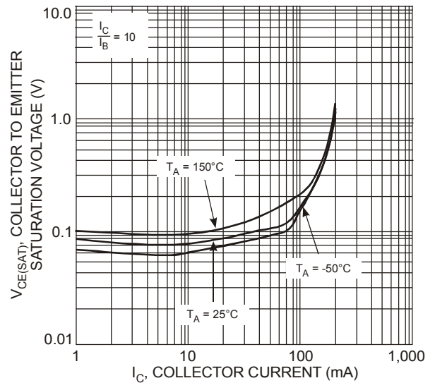
Fig. 6, Collector Emitter Saturation Voltage vs. Collector Current (PNP5401)
