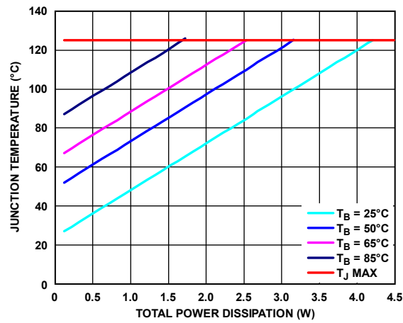
Figure 61. LFCSP Junction Temperature Rise, Different Board Temperatures
