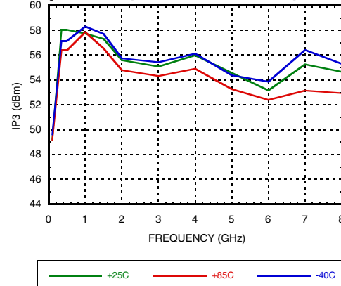
Input Third Order Intercept Point over Temp., 3.3V (100 MHz - 8 GHz)
